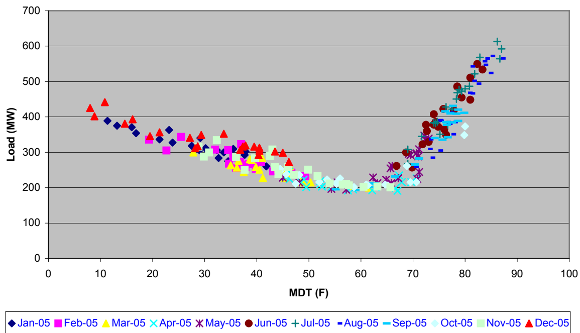
Average Residential Class Load vs. MDT
