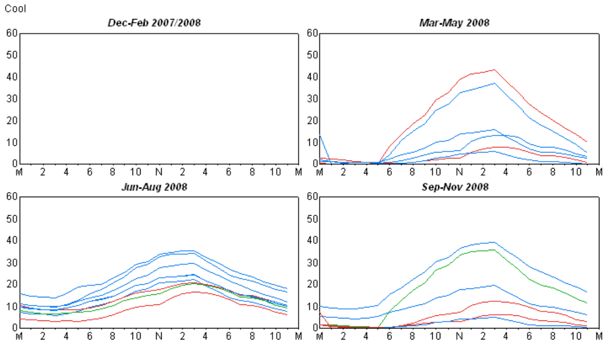
Figure 7: SJ Large General Service Air Conditioning Profile
