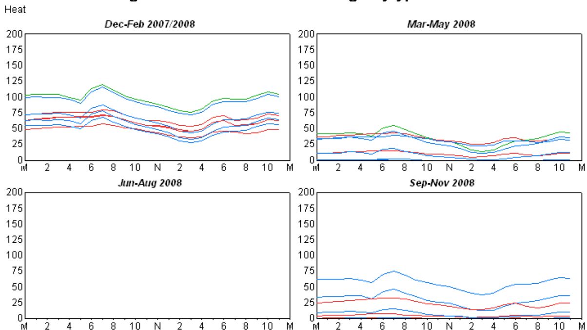
Figure 2: SJ Residential Heating Daytype Profile
