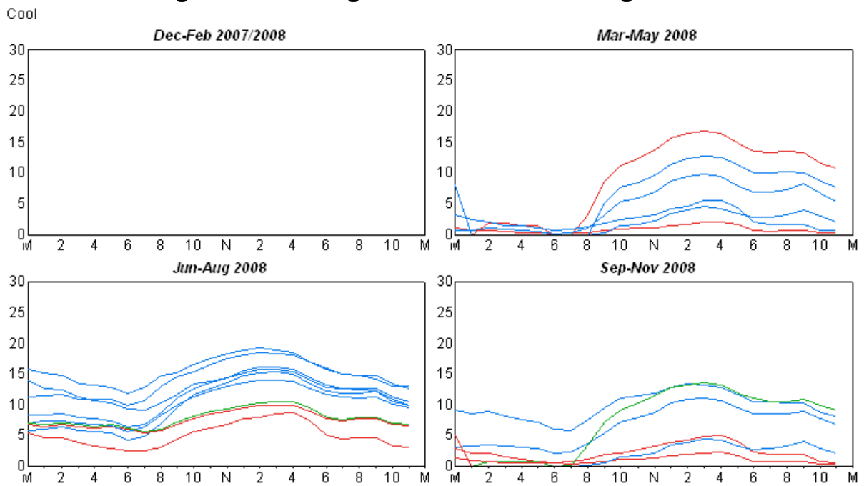
Figure 10: SJ Large Power Air Conditioning Profile
