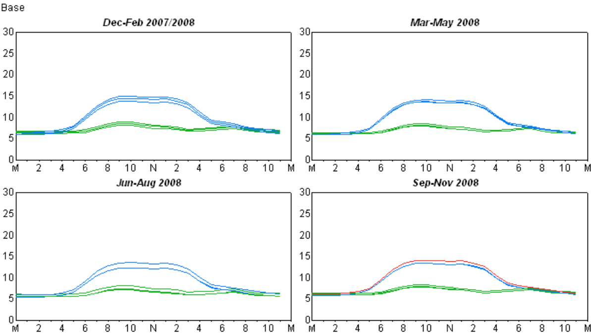
Figure 6: SJ Small General Service Other Profile
