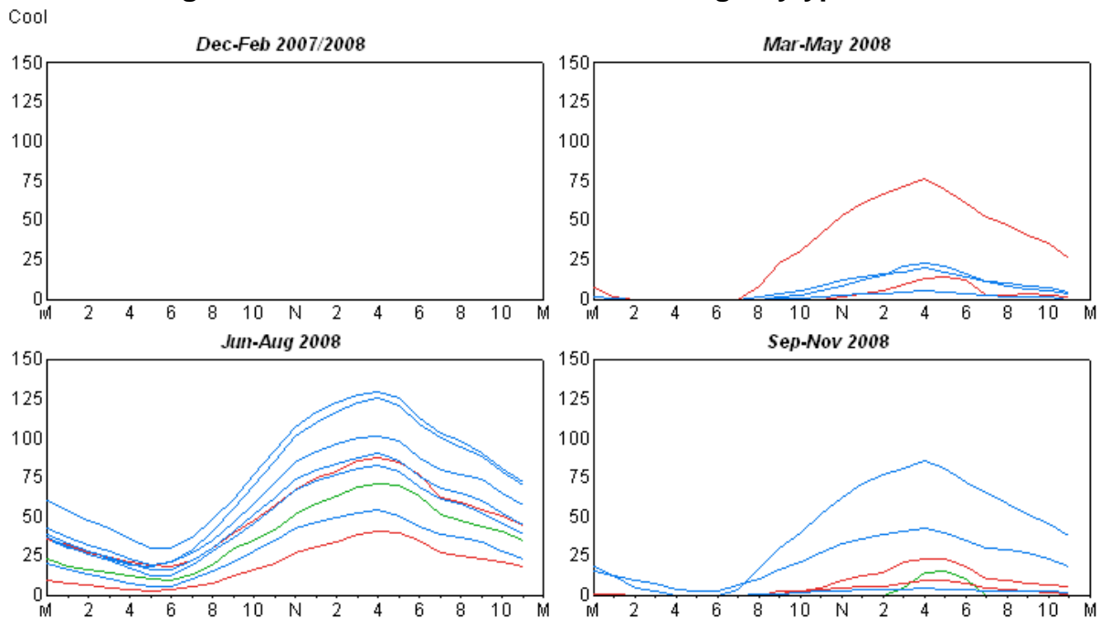
Figure 1: SJ Residential Air Conditioning Daytype Profile
