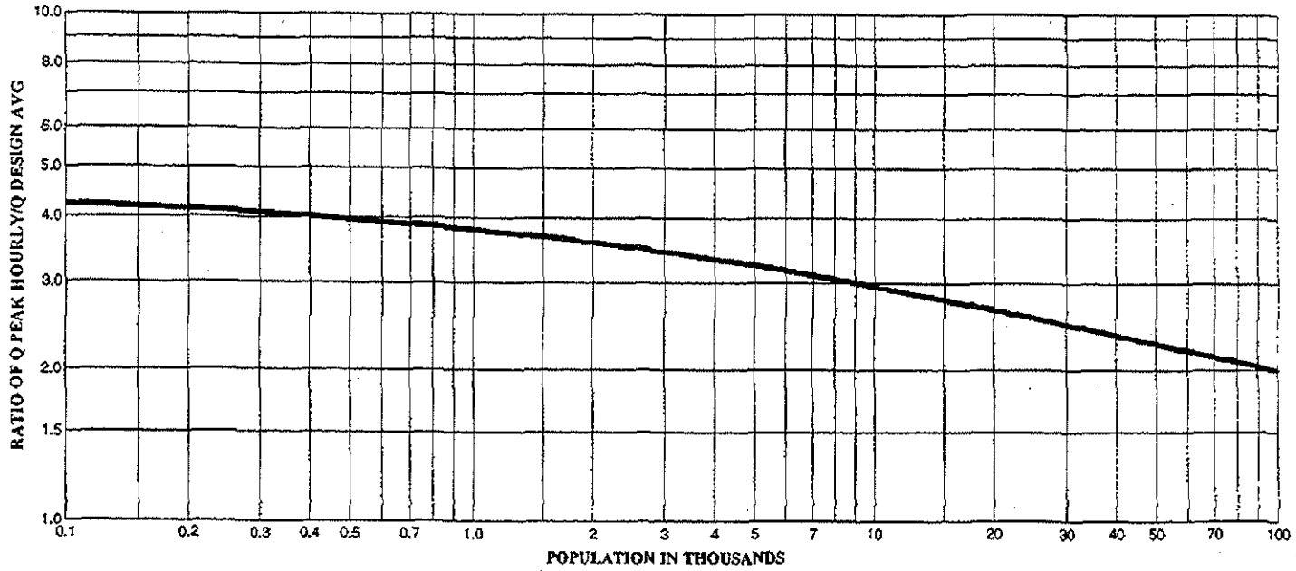
Figure 1. Ratio of peak hourly flow to design average flow.
