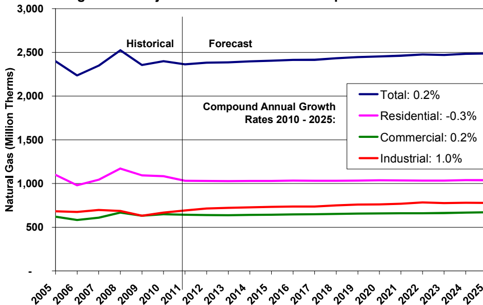
Figure 10. Projected Natural Gas Consumption 2010–2025
