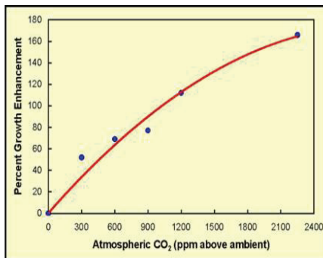
Figure 3. Positive Impact of CO 2 on Plants and Trees. Adapted from Idso, K.E. (1992).
