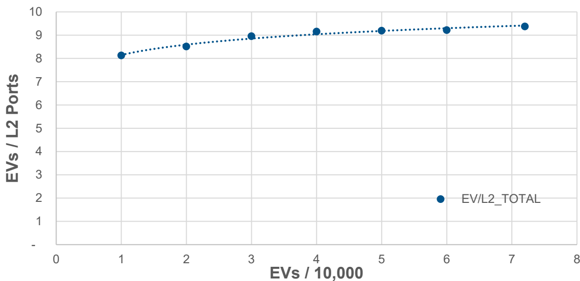
Figure 3. Level 2 Ports as a Function of EVs in Evergy's Missouri West Service Territory
